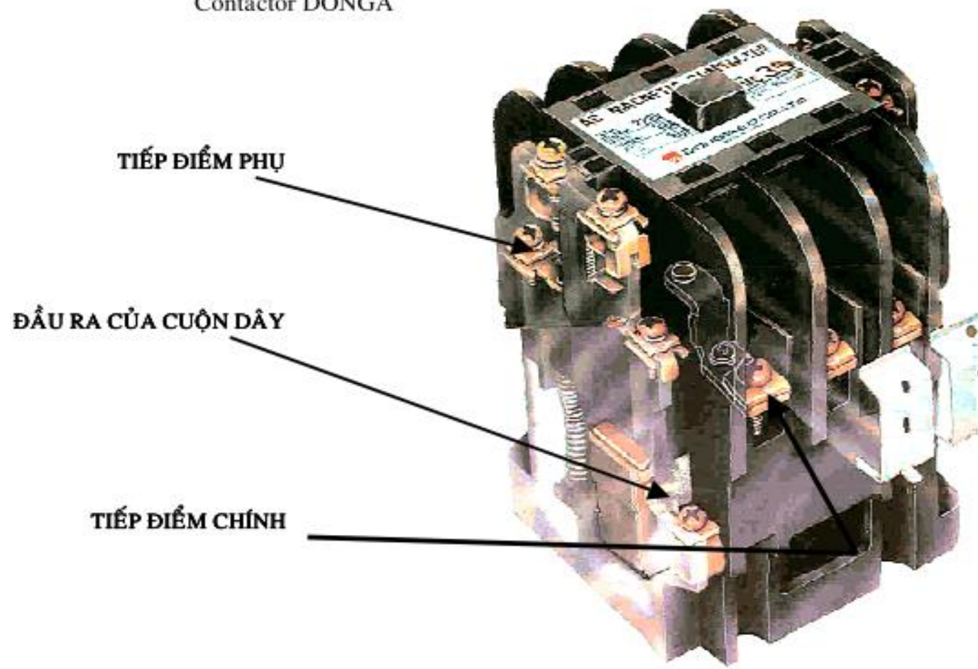
Contactor DONGA
